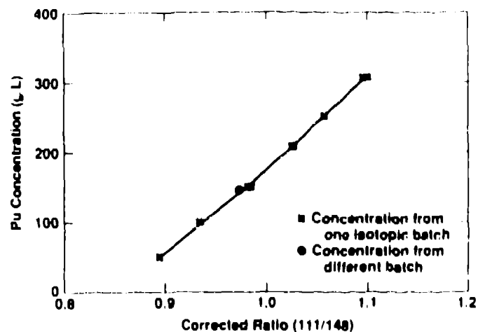
Fig. 4. The plutonium concentration as a function of the measured 111/148 ratios after the isotopic correction.
